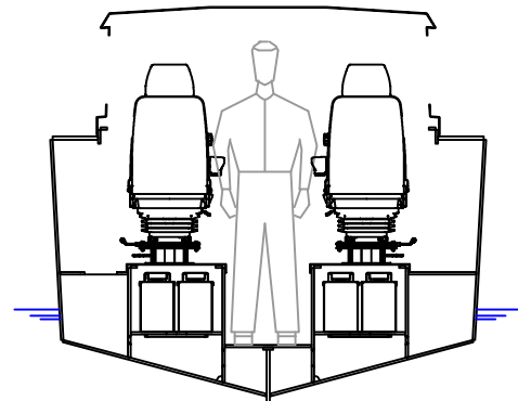
CROSS SECTION FR12
